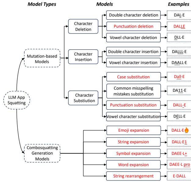
Figure 3: The 14 kinds of squatting-generation models used in this work. The 6 models in black are inherited from AppCrazy [24], while the 8 models in red that are either newly introduced or modified in LLMappCrazy to target LLM apps.
