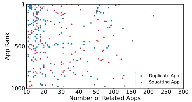
Figure 7: Distribution of fake and squatting apps by app rank.
