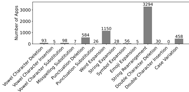
Figure 6: The distribution of squatting apps across models.
