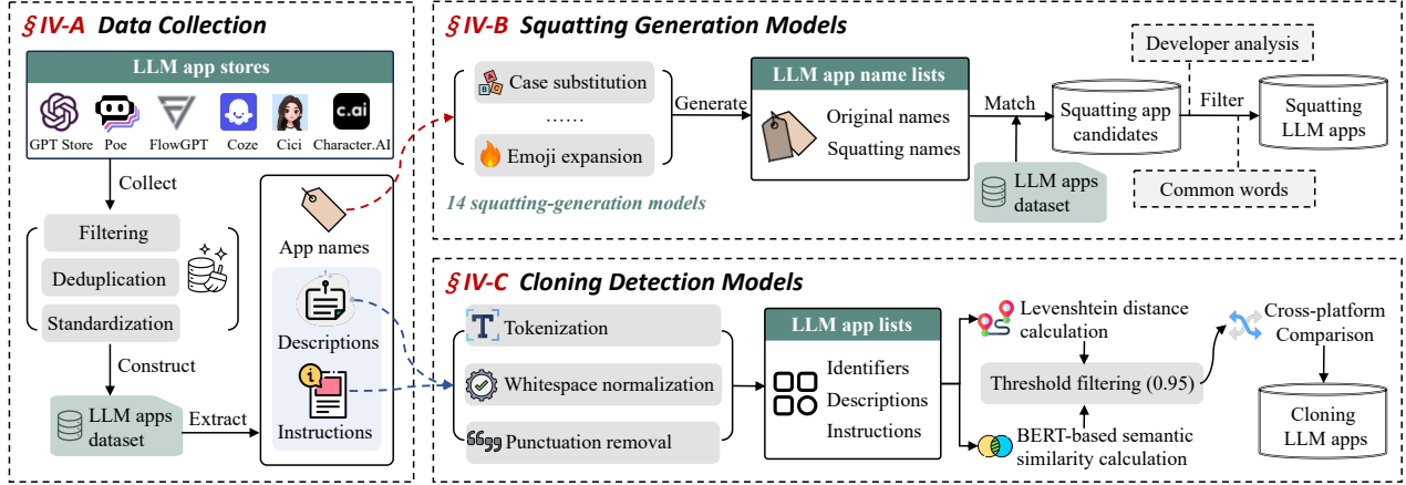
Figure 2: Our approach to identifying squatting and cloning LLM apps.
