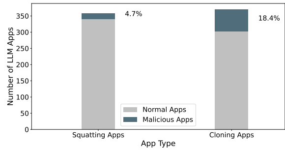
Figure 9: Result of sampling analysis.
